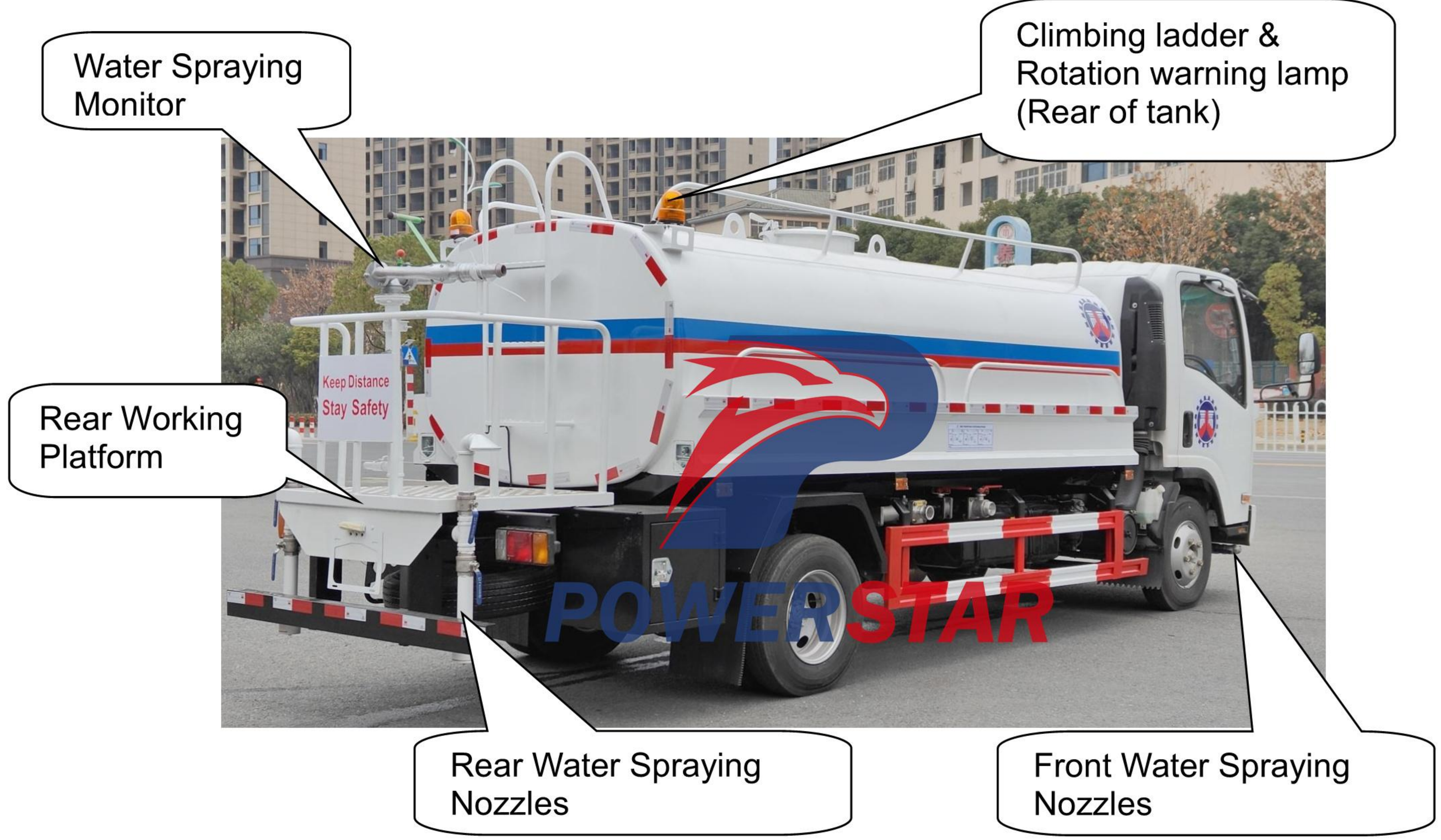
Rear of the Tank: Climbing ladder, water spraying monitor and nozzles.
